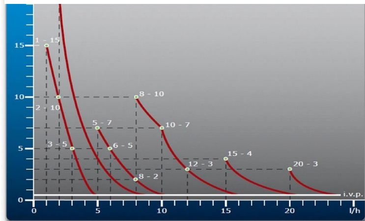
Pressure (bar) – Flow Rate (l/h) Chart
