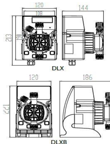
Overall Dimensions
